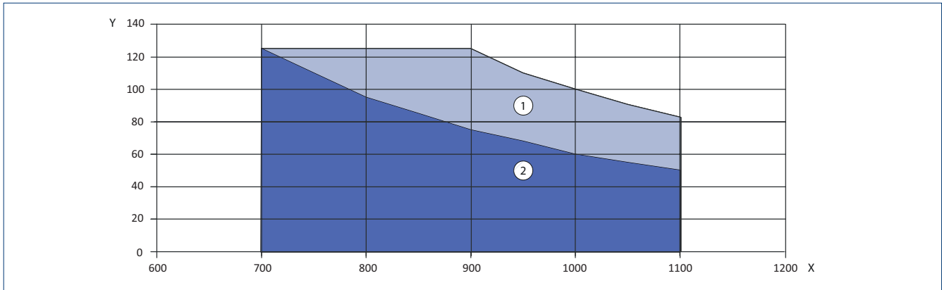
X = Door width (mm) | Y = Door weight (kg) | 1 = Area of application in low-energy mode | 2 = Area of application in automatic mode | Minimum door width for installation in metal door or frame 750 mm
