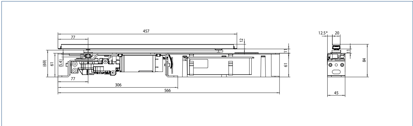
ECTurn Inside Representation of a wooden door leaf, mirror-inverted for door frames
