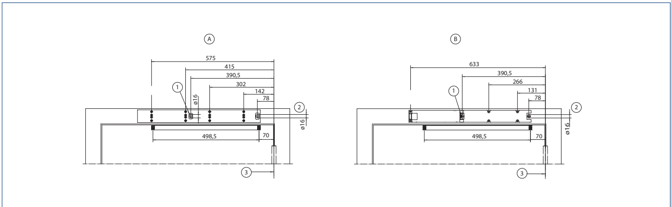
A = Installation with mounting plate | B = Direct installation | 1 = Concealed line-feed for low-voltage connection | 2 = Concealed line-feed for low-voltage connection and mains cable | 3 = Dimensional reference centre of hinge
