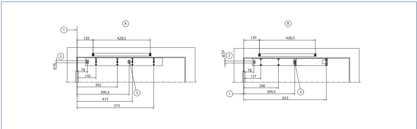
A = Installation with mounting plate | B = Direct installation | 1 = Dimensional reference centre of hinge | 2 = Concealed line-feed for low-voltage connection and mains cable | 3 = Concealed line-feed for low-voltage connection
