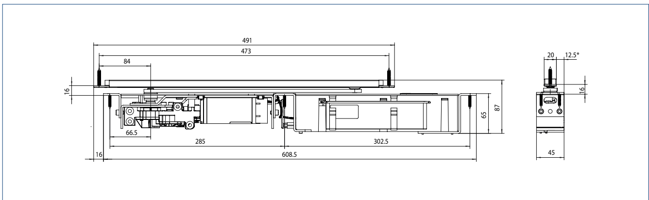
ECTurn Inside Representation of a metal door leaf, mirror-inverted for door frames
