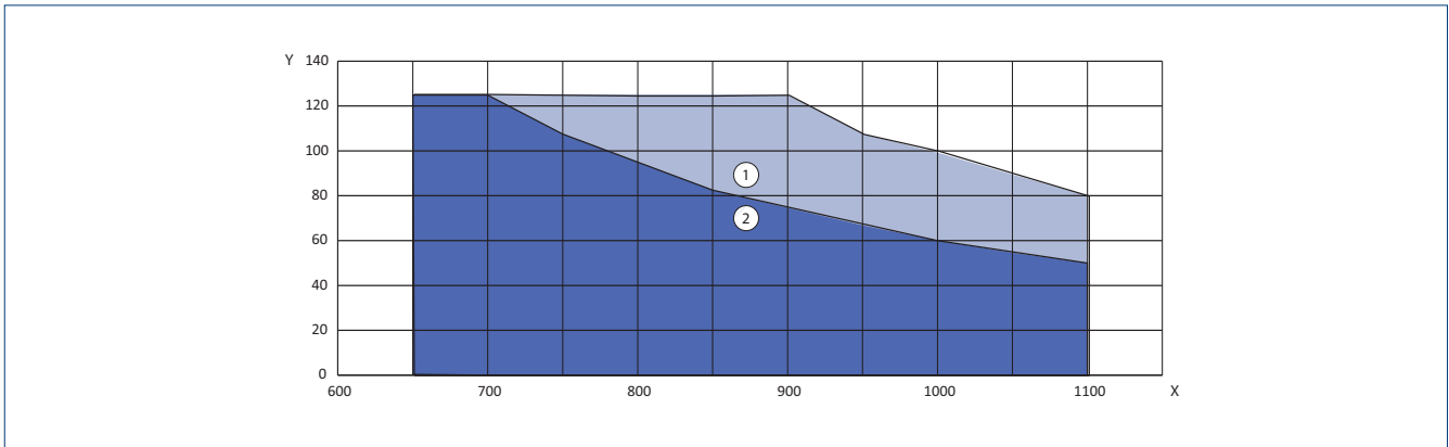
X = Door width (mm) | Y = Door weight (kg) | 1 = Area of application in low-energy mode | 2 = Area of application in automatic mode
