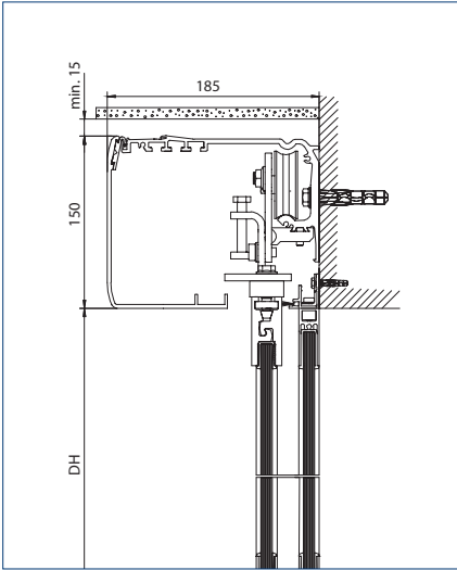
Door system with door leaf and side screens under drive
