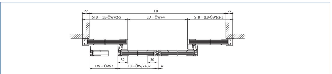
Installation: Wall installation with girder section
