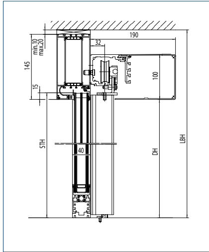
Vertical section side screen, angled floor guide
