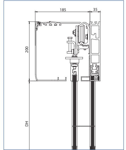
Door system with door leaf and side screens under girder section
